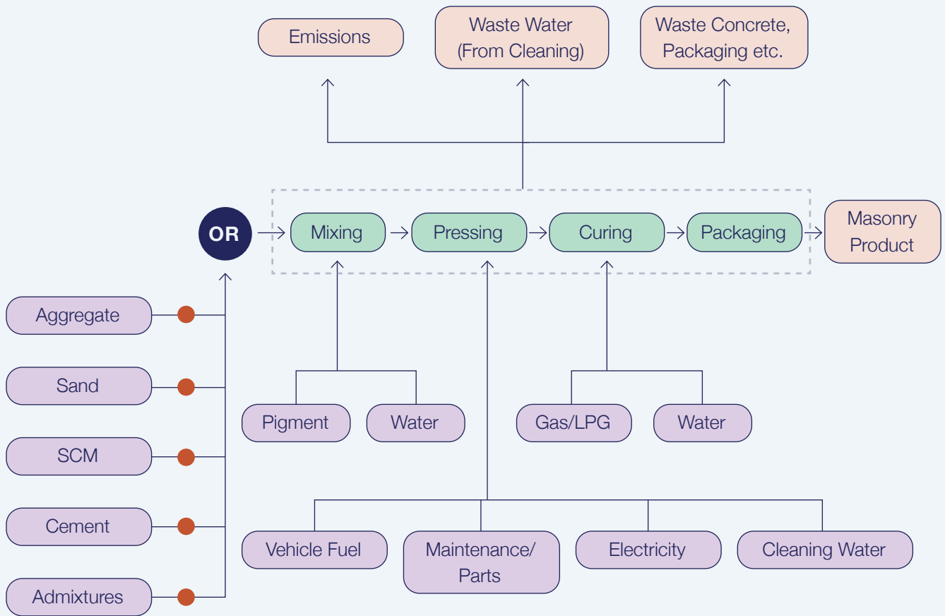
Figure 1 | Typical process flow for an Adbri Masonry plant
