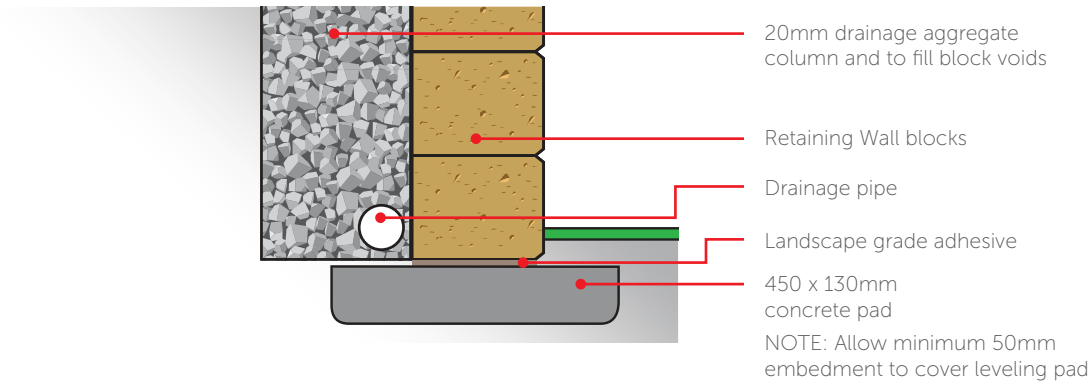
CONCRETE LEVELLING PAD FOOTING
