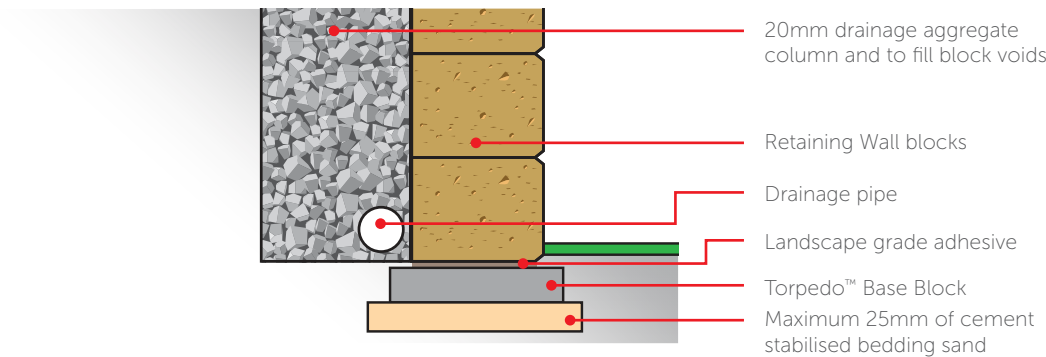
TORPEDO™ BASE BLOCK FOOTING
