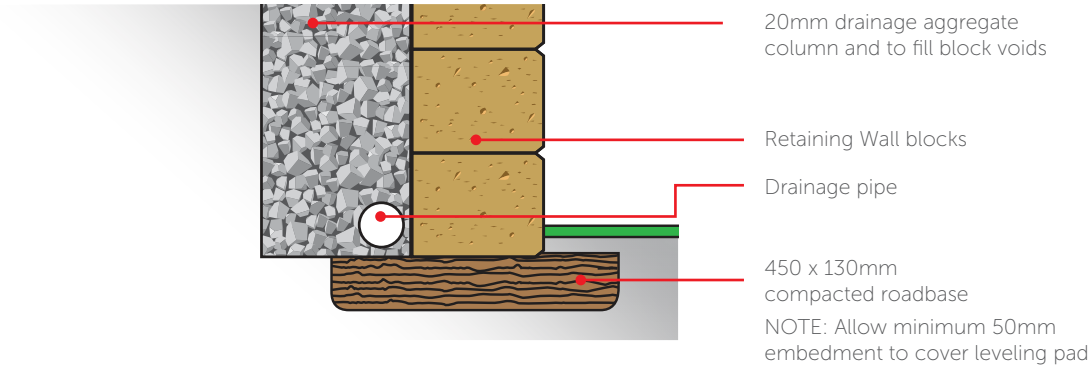
COMPACTED ROADBASE FOOTING
